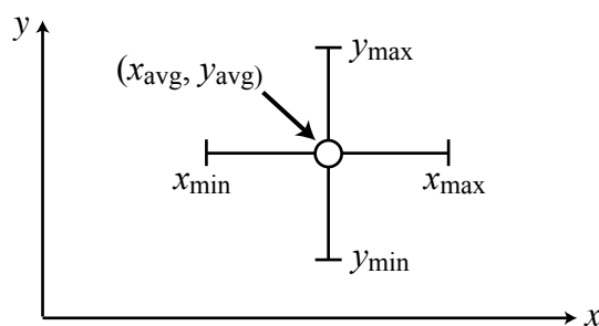
Figure 13.1. Diagram of error bars showing uncertainties in the value of the x - and y -coordinates and point (x_{avg}, y_{avg}) .
