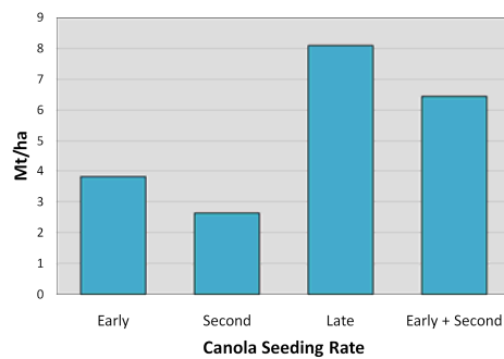
Fig 2: Effect of Cut Date on Forage Yield
