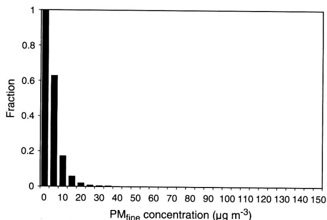
Fig. 3. Cumulative frequency distribution of PM fine concentrations at Kennewick, WA from 1999 through 2005. Daily PM concentrations, categorized by 5\text{-}\mu\text{g m}^{-3} intervals, were measured by a federal reference method filter-based sampler or tapered element oscillating microbalance.
