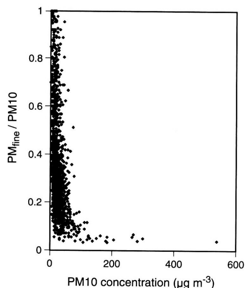
Fig. 4. PM fine /PM 10 ratio as a function of daily PM 10 concentration from 1999 through 2005 at Kennewick, WA.
