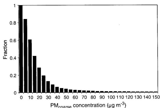
Fig. 5. Cumulative frequency distribution of PM coarse concentrations at Kennewick, WA from 1999 through 2005. Daily PM concentrations, categorized by 5- \mu\text{g m}^{-3} intervals, were determined using federal reference method filter-based samplers or tapered element oscillating microbalances.
