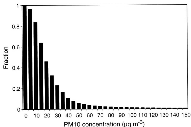
Fig. 2. Cumulative frequency distribution of \text{PM}_{10} concentrations at Kennewick, WA from 1999 to 2005. Daily \text{PM} concentrations, categorized by 5\text{-}\mu\text{g m}^{-3} intervals, were measured by a federal reference method filter-based sampler or tapered element oscillating microbalance.
