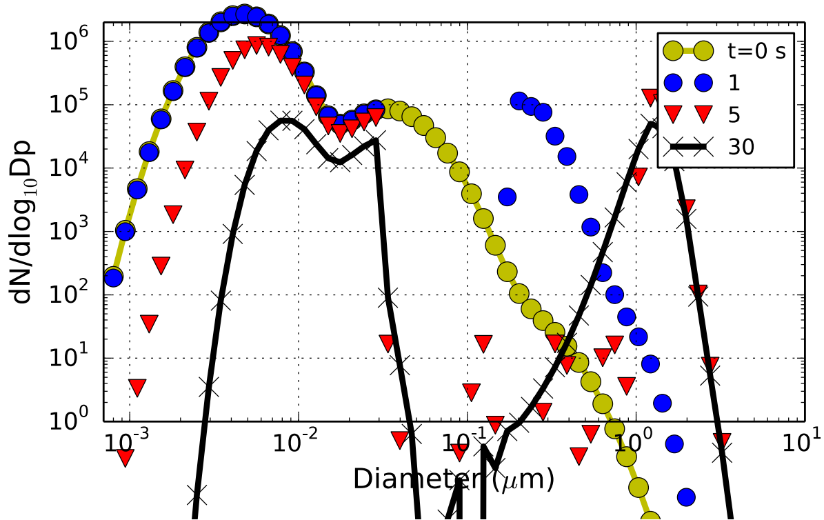
Figure 4. The base case aerosol size distribution ( N = \#/\text{cm}^3 ) at initialization (0 s) and after 1, 5, and 30 seconds using GATOR-GCMOM. Aerosol composition includes black carbon (BC), primary organic matter (POM), sulfate [S (VI)], and water vapor ( \text{H}_2\text{O} ).
