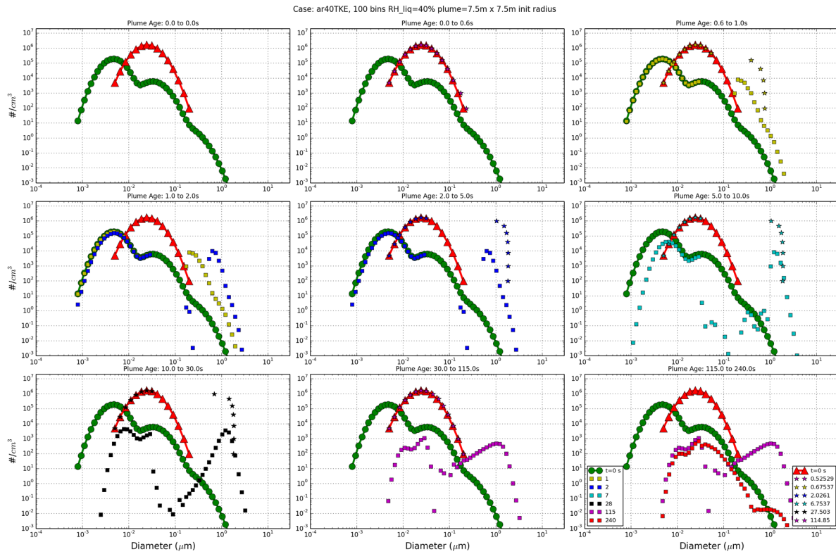
Figure 13. Comparison of GATOR-GCMOM (squares) and Aerodyne (stars) modeled number concentrations ( \#/\text{cm}^3 ) at 40% ambient relative humidity. Initial distributions for GATOR-GCMOM (green circles) and Aerodyne (red triangles) are also shown in each panel.
