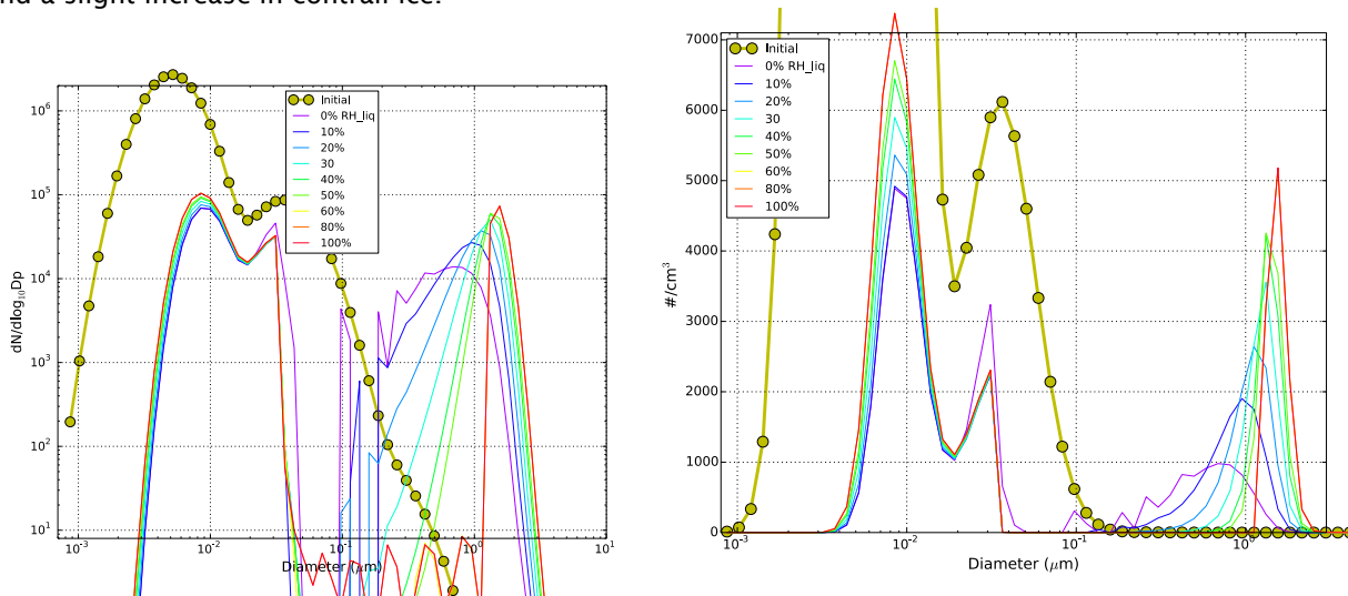
Figure 6. Aerosol size distribution after 23 seconds for simulations with varying ambient relative humidity (RH-liquid) using GATOR-GCMOM. Number concentration ( N = \#/\text{cm}^3 ) is normalized by size bin diameter ( D_p ) in the left figure.
