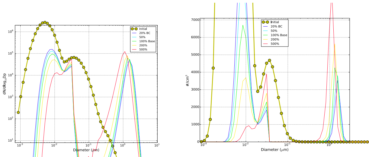
Figure 8. Aerosol size distribution after 23 seconds for simulations using GATOR-GCMOM that vary the BC emission index. Number concentration ( \#/cm^3 ) is normalized by size bin diameter ( D_p ) in the left figure.
