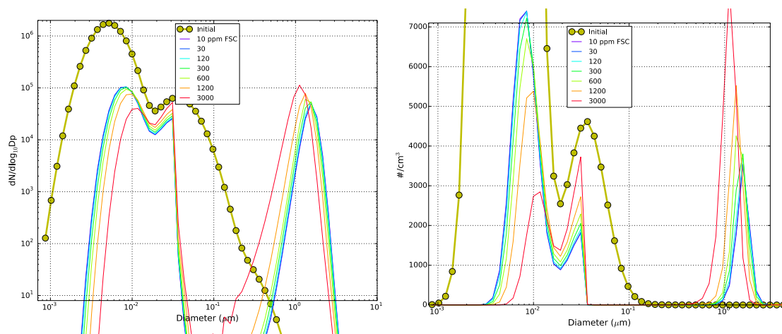
Figure 10. Aerosol size distribution after 23 seconds for simulations using GATOR-GCMOM that vary the fuel sulfur content. Number concentration ( \#/cm^3 ) is normalized by size bin in the left figure. The base case uses a FSC of 600 ppm.
