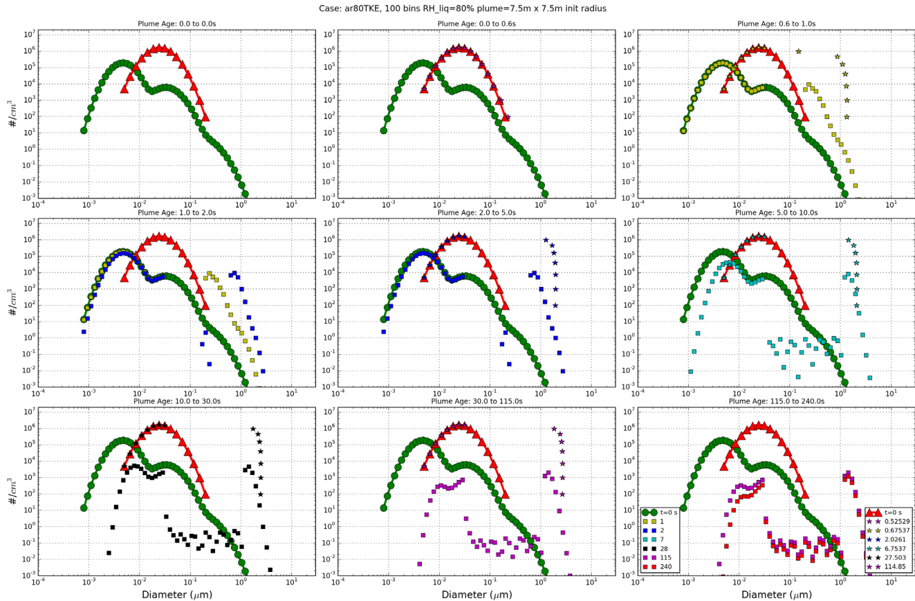
Figure 14. Comparison of GATOR-GCMOM (squares) and Aerodyne (stars) modeled number concentrations ( \#/cm^3 ) at 80% ambient relative humidity. Initial distributions for GATOR-GCMOM (green circles) and Aerodyne (red triangles) are also shown in each panel.
