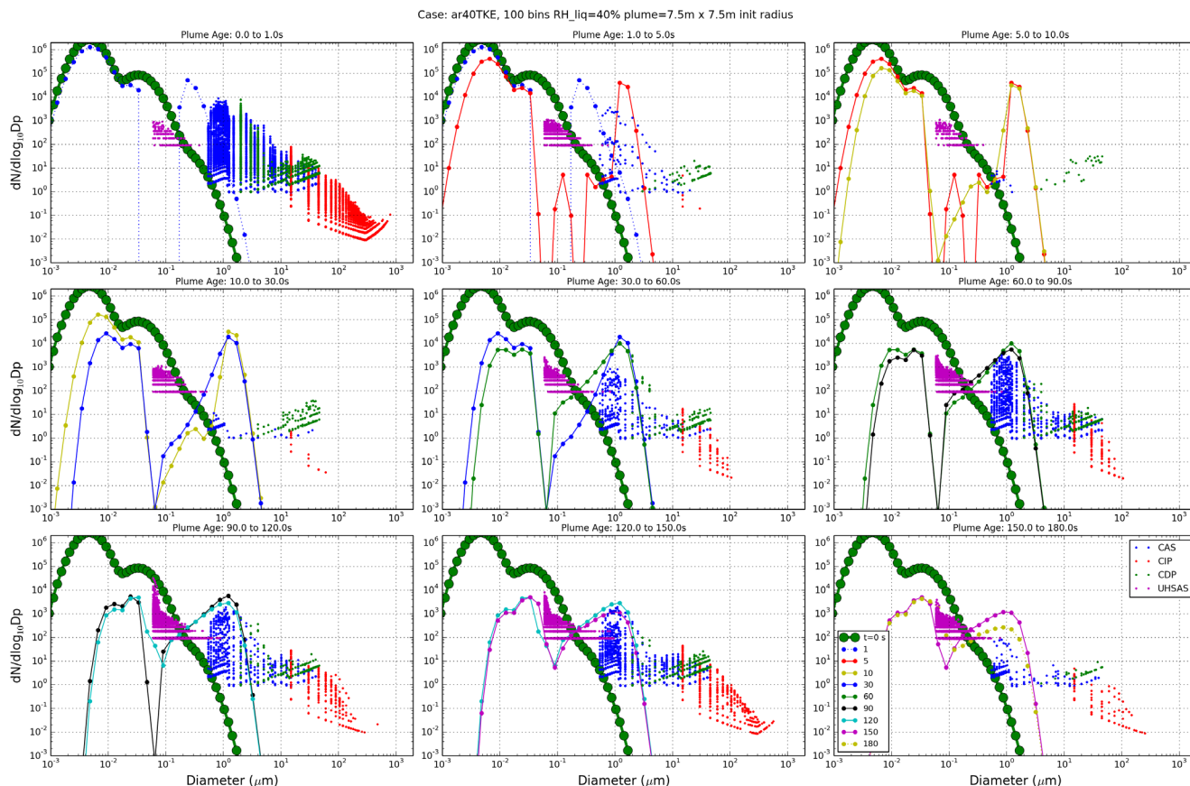
Figure 12. Measured contrail size distributions for the May 29, 2014 ACCESS 2 flight, filtered and separated by plume age. GATOR-GCMOM model results at t=0, 1, 5, 10, 30, 60, 90, 120, 150, and 180 s are also shown in panels with data of the same age.
