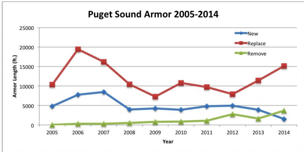
New, replaced, and removed Puget Sound armoring (2005-2014). Source: WDFW
