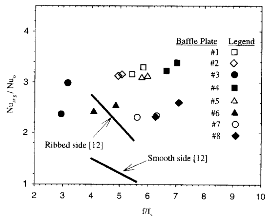
Fig. 10. Qualitative performance comparison of baffles with ribbed channel [12].
