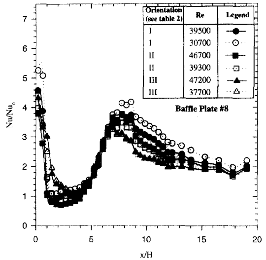
Fig. 7. Local Nusselt number ratio distribution along the channel centerline for Baffle Plate 8 at different angles.
